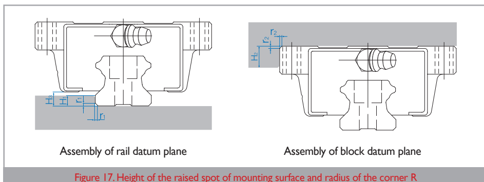
Figure 17. Height of the raised spot of mounting surface and radius of the corner R
