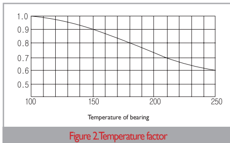
Figure 2. Temperature factor
