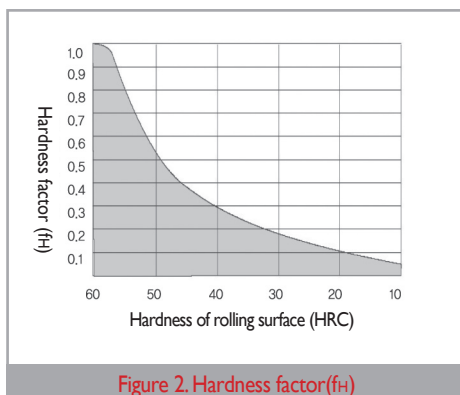
Figure 2. Hardness factor( f_H )
