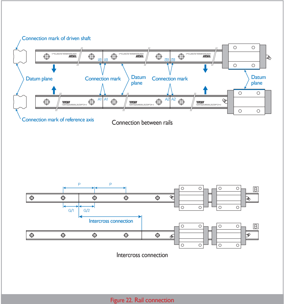
Figure 22. Rail connection
