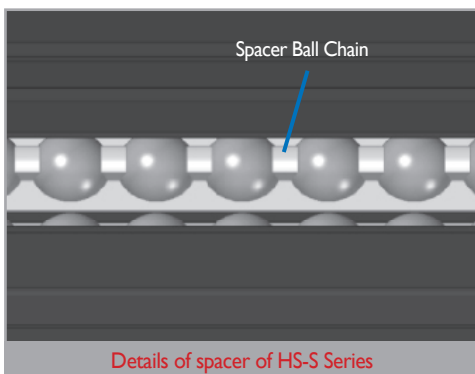
HS...S Series (Spacer Chain Type)
