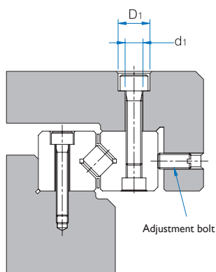
Figure 3. An example of preload adjustment
