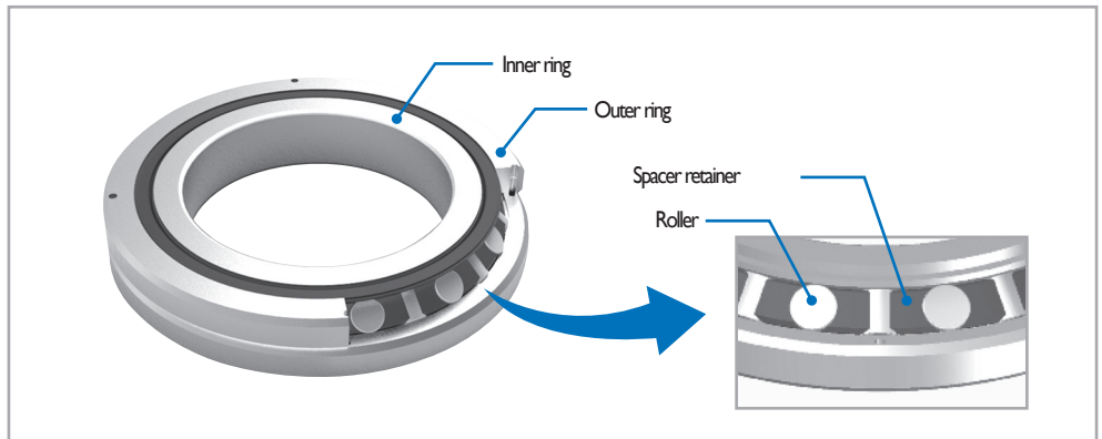
Figure I. Structure of Crossed Roller Bearing
