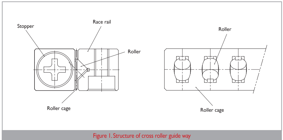
Figure 1. Structure of cross roller guide way
