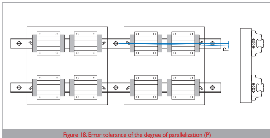
Figure 18. Error tolerance of the degree of parallelization (P)
