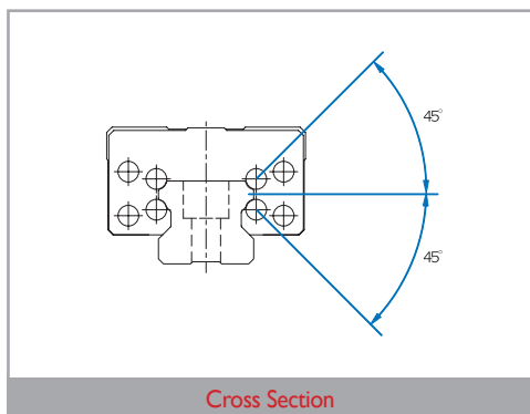
HS Series (Full Ball Type)
